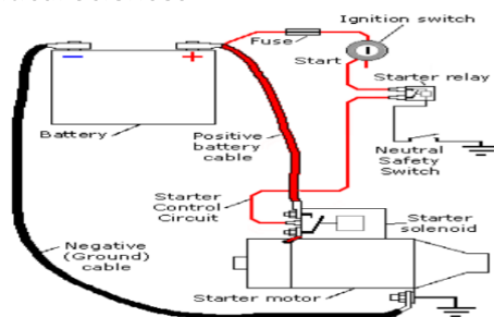
Figure.1. Starting system of electronic ignition
