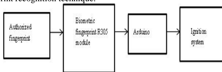
Figure.2. Block diagram of vehicle anti-theft system
