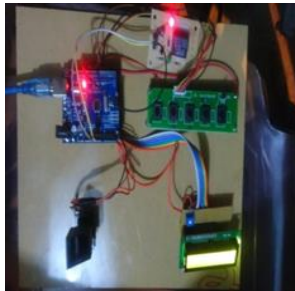
Figure.7. Unauthorized person fingerprint is scanned and the engine remains off
