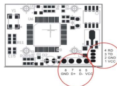
Figure.3. R305 Fingerprint module
