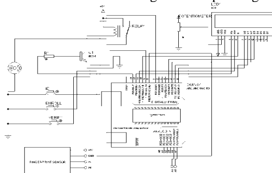
Figure.4. Interface between ignition system and microcontroller
