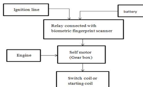
Figure.5. Engine system with hardware connected to the vehicle engine starting system
