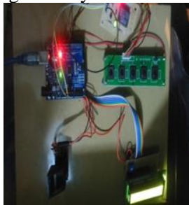
Figure.6. Authorized person fingerprint is scanned and the engine turned on
