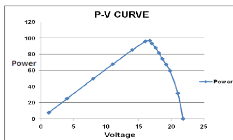
Figure.3. Power-Voltage characteristics of PV Solar system
