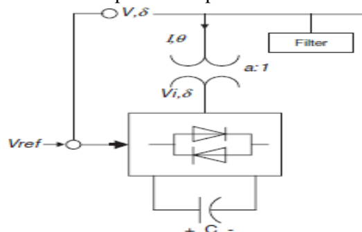
Figure.1. STATCOM Structure
