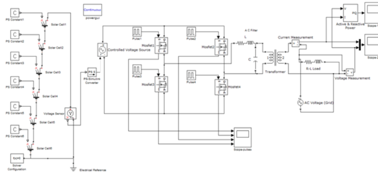
Figure.6. MATLAB simulation with PV solar controller as a STATCOM
