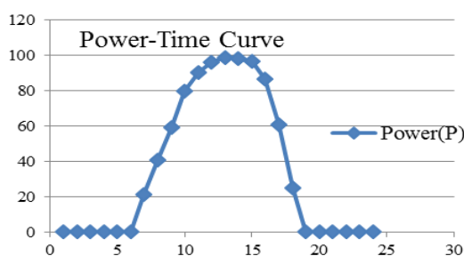
Figure.4. Power-Time characteristics of PV Solar system
