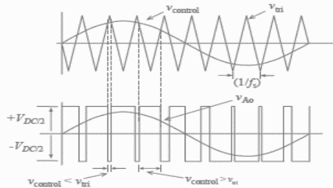
Figure.2. PWM for firing of converter valves
