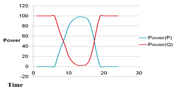
Figure.5. Real and Reactive power exchange characteristics of PV Solar system
