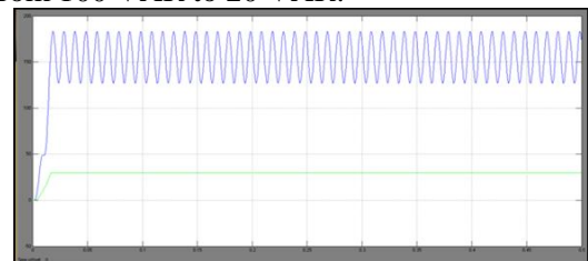
Figure.10. Active Reactive power with PV solar controller as a STATCOM
